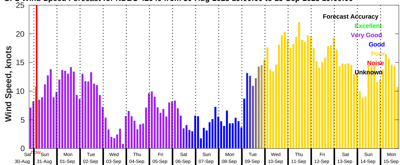
GFS Wind Speed Forecast for NDBC 42040 from 30-Aug-2025 19:00:00 to 15-Sep-2025 19:00:00
