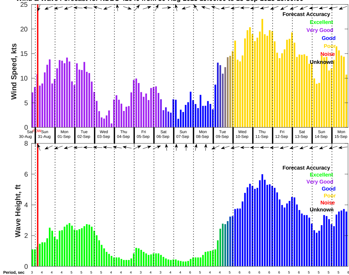
Wind & Wave Forecast for NDBC 42040 from 30-Aug-2025 19:00:00 to 15-Sep-2025 19:00:00
