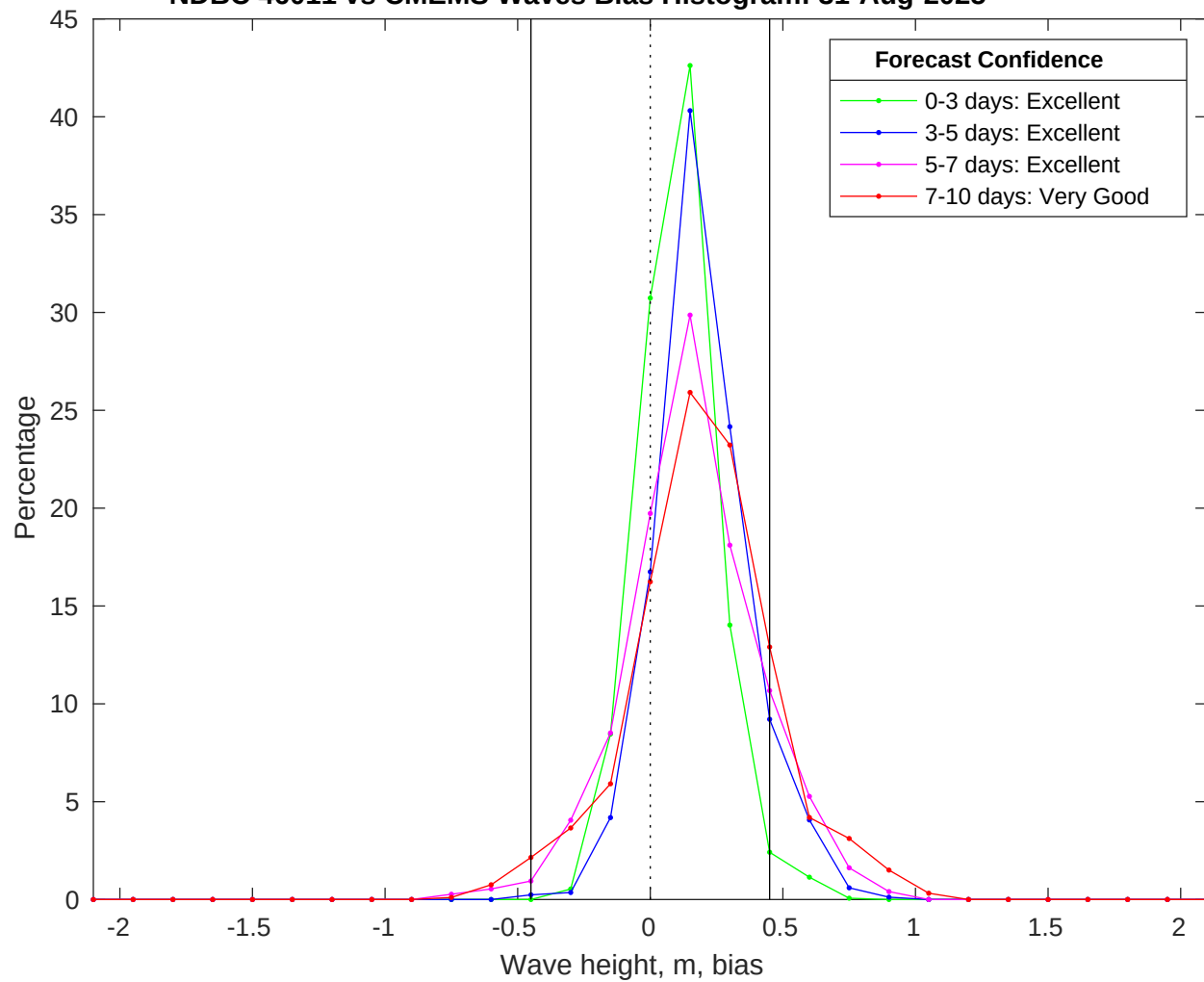
NDBC 46011 vs CMEMS Waves Bias Histogram: 31-Aug-2025
