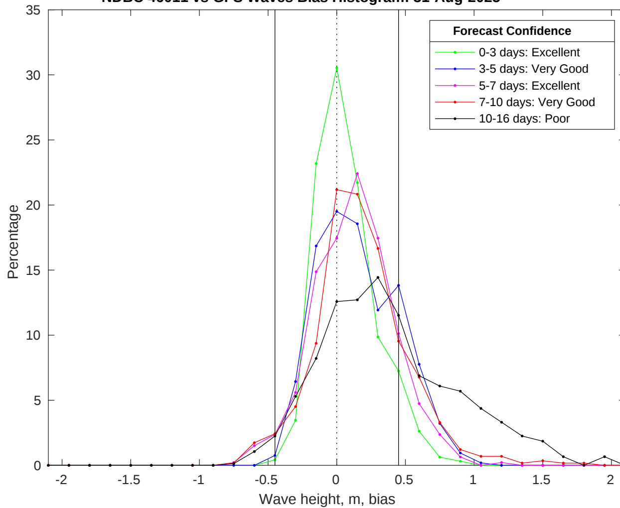
NDBC 46011 vs GFS Waves Bias Histogram: 31-Aug-2025
