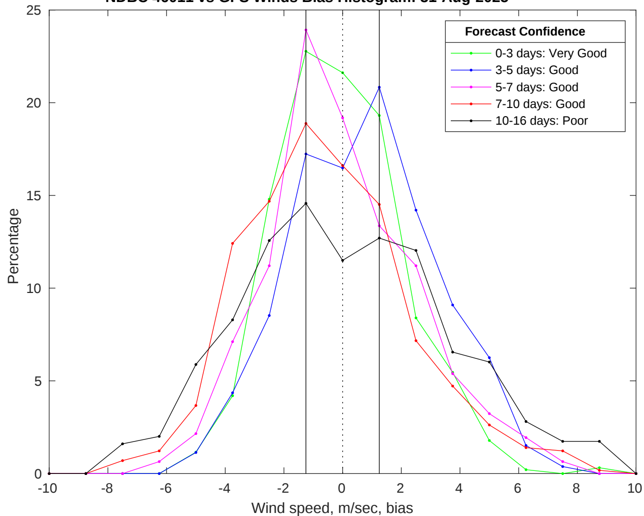
NDBC 46011 vs GFS Winds Bias Histogram: 31-Aug-2025
