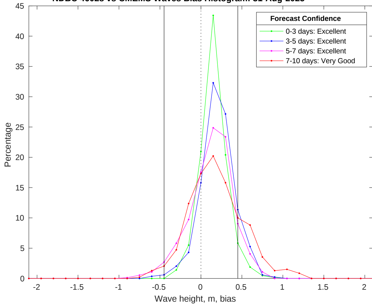
NDBC 46028 vs CMEMS Waves Bias Histogram: 31-Aug-2025
