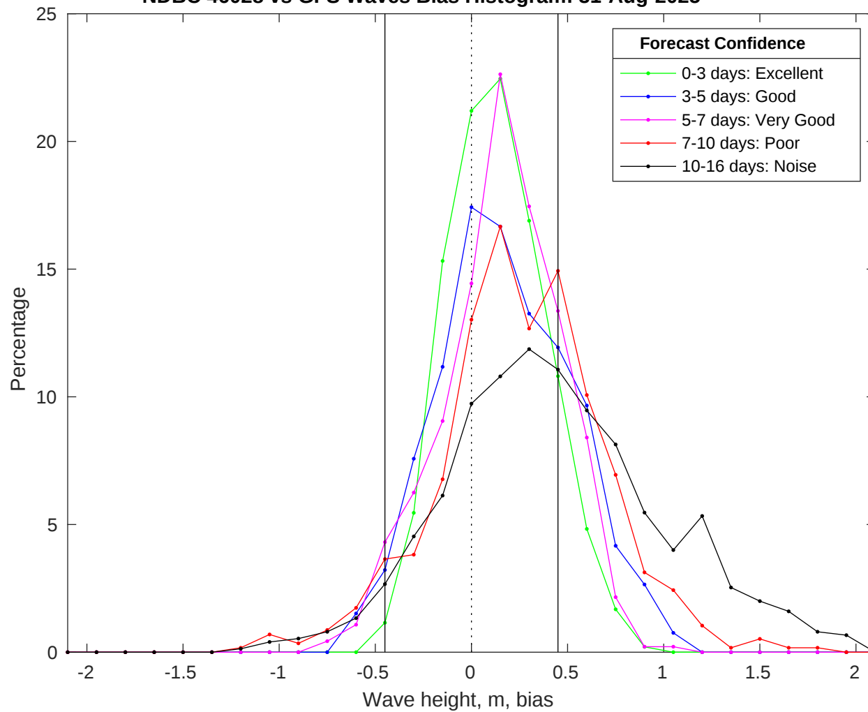
NDBC 46028 vs GFS Waves Bias Histogram: 31-Aug-2025
