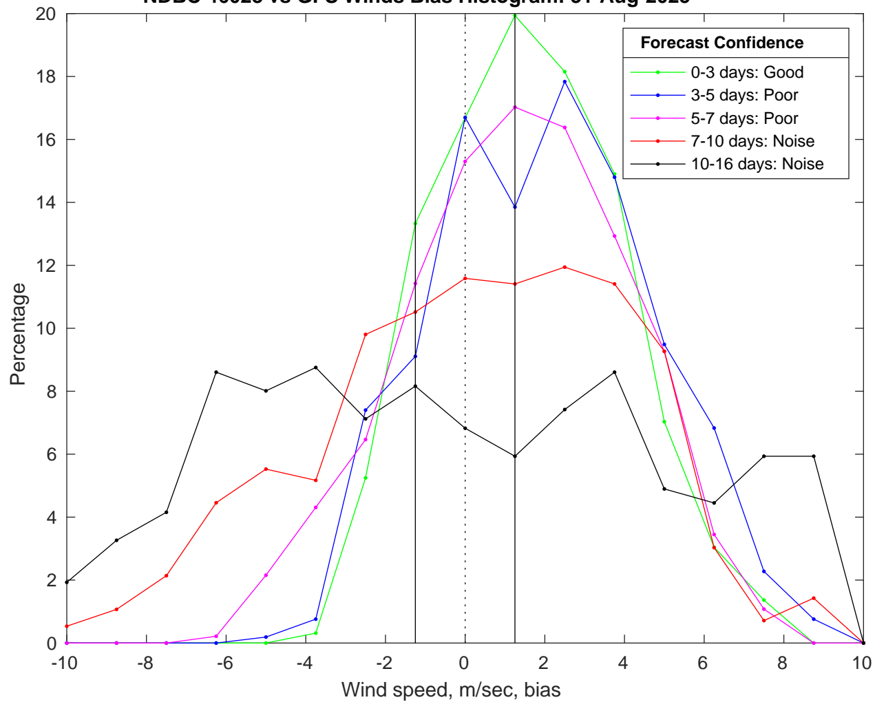
NDBC 46028 vs GFS Winds Bias Histogram: 31-Aug-2025
