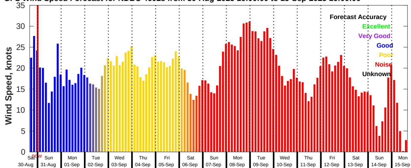
GFS Wind Speed Forecast for NDBC 46028 from 30-Aug-2025 16:00:00 to 15-Sep-2025 16:00:00
