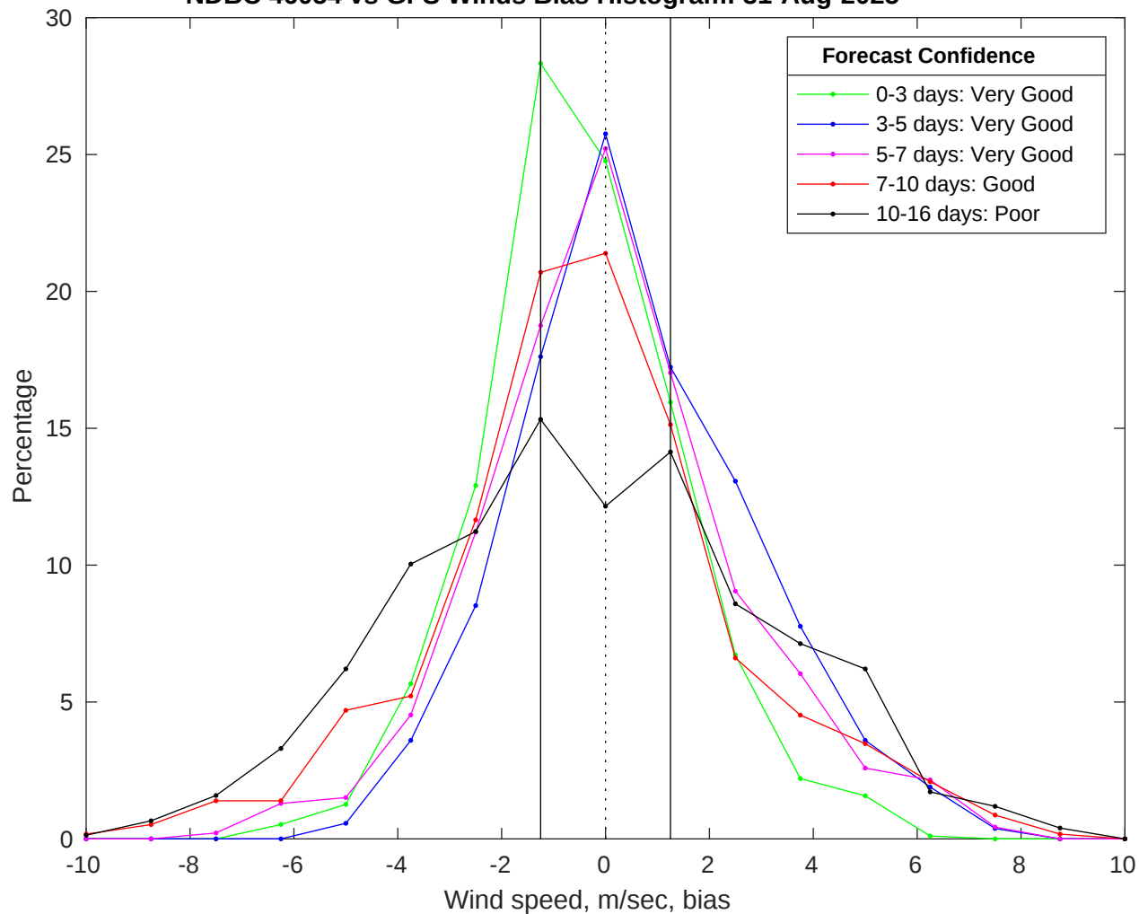
NDBC 46054 vs GFS Winds Bias Histogram: 31-Aug-2025
