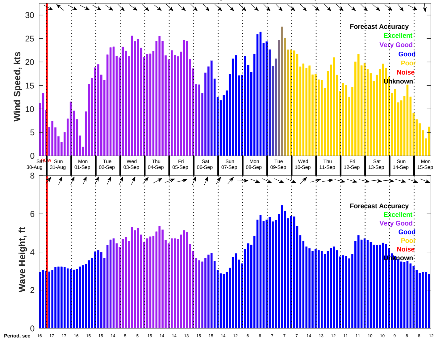
Wind & Wave Forecast for NDBC 46054 from 30-Aug-2025 16:00:00 to 15-Sep-2025 16:00:00
