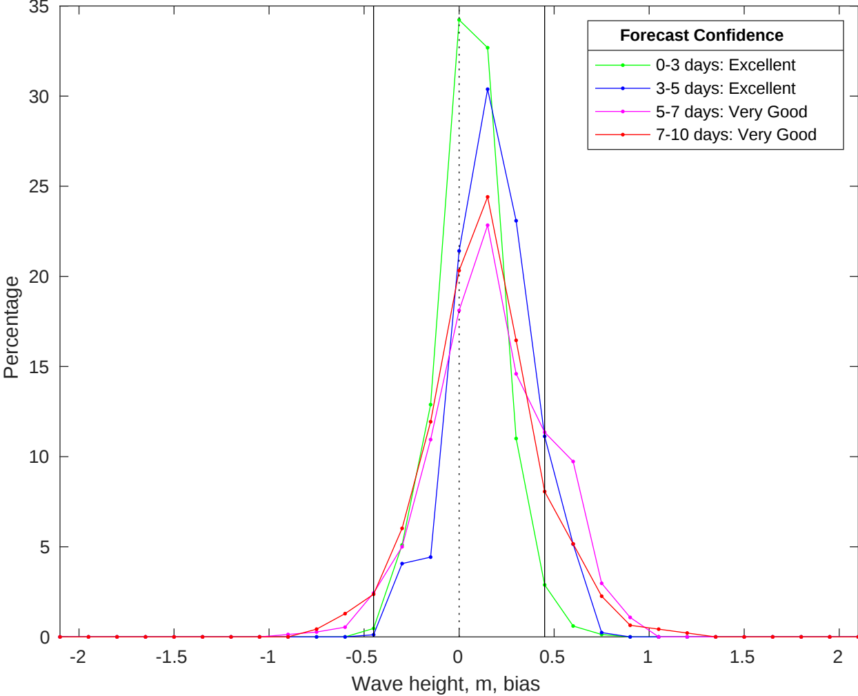
NDBC 46069 vs CMEMS Waves Bias Histogram: 31-Aug-2025
