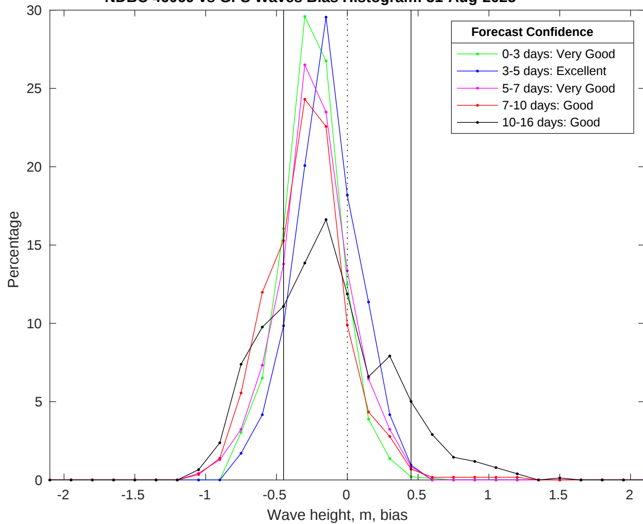
NDBC 46069 vs GFS Waves Bias Histogram: 31-Aug-2025
