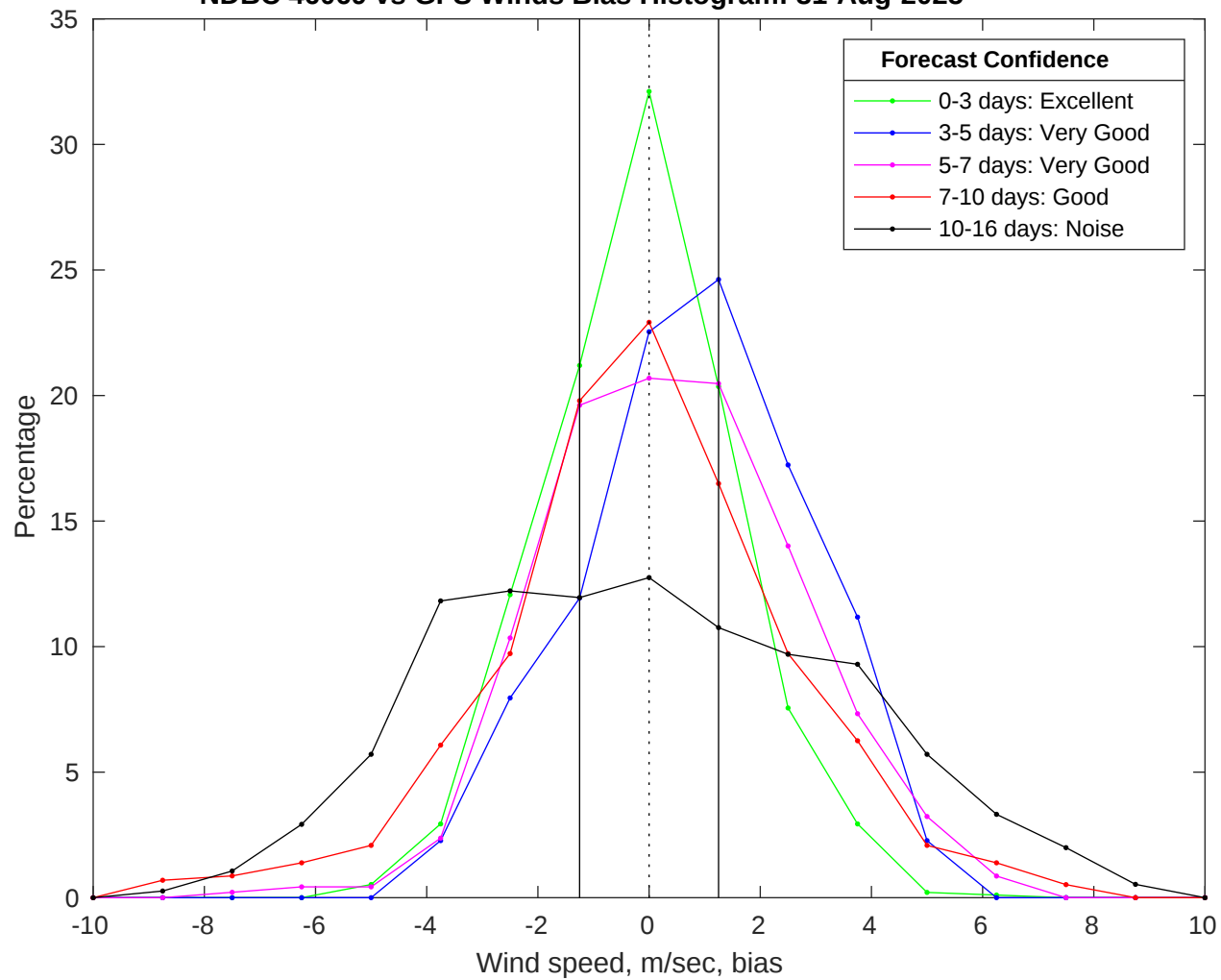
NDBC 46069 vs GFS Winds Bias Histogram: 31-Aug-2025
