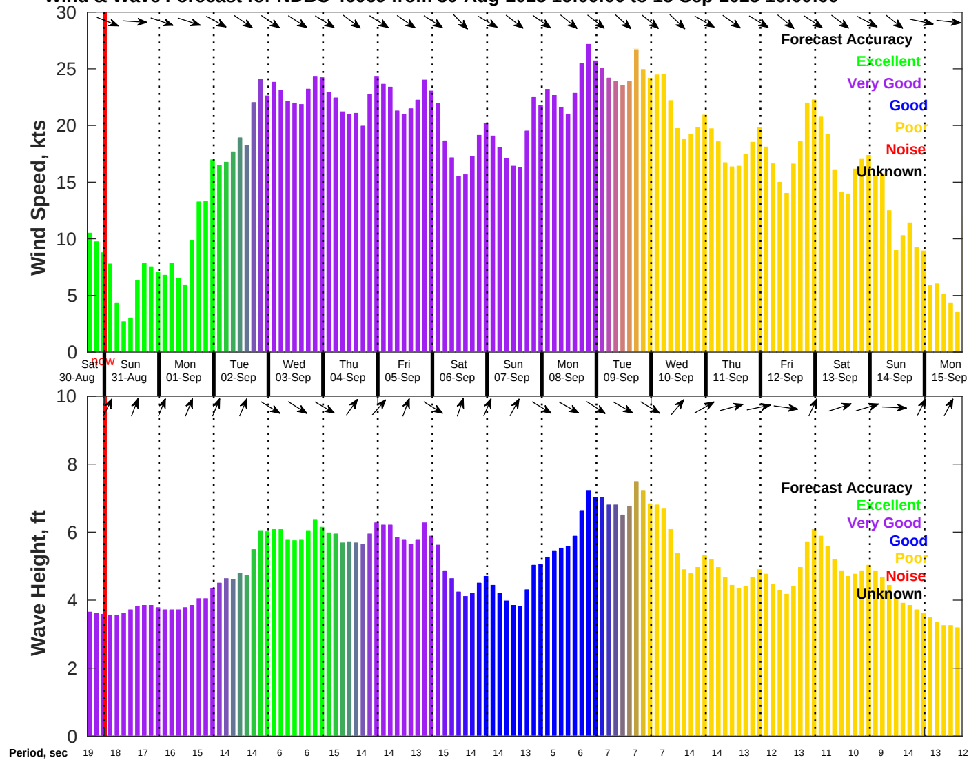
Wind & Wave Forecast for NDBC 46069 from 30-Aug-2025 16:00:00 to 15-Sep-2025 16:00:00
