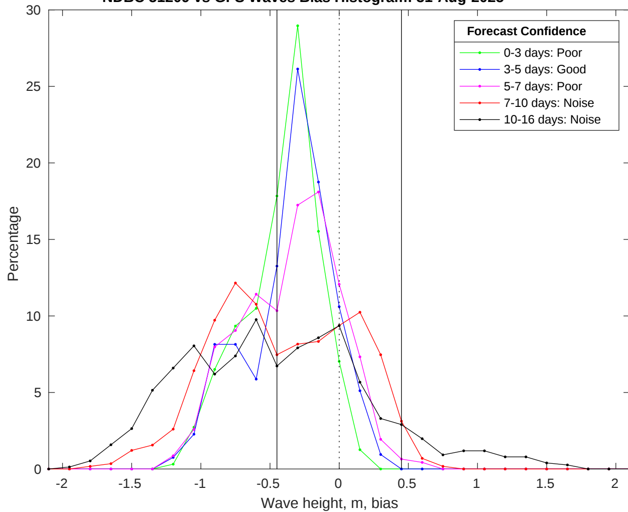
NDBC 51209 vs GFS Waves Bias Histogram: 31-Aug-2025
