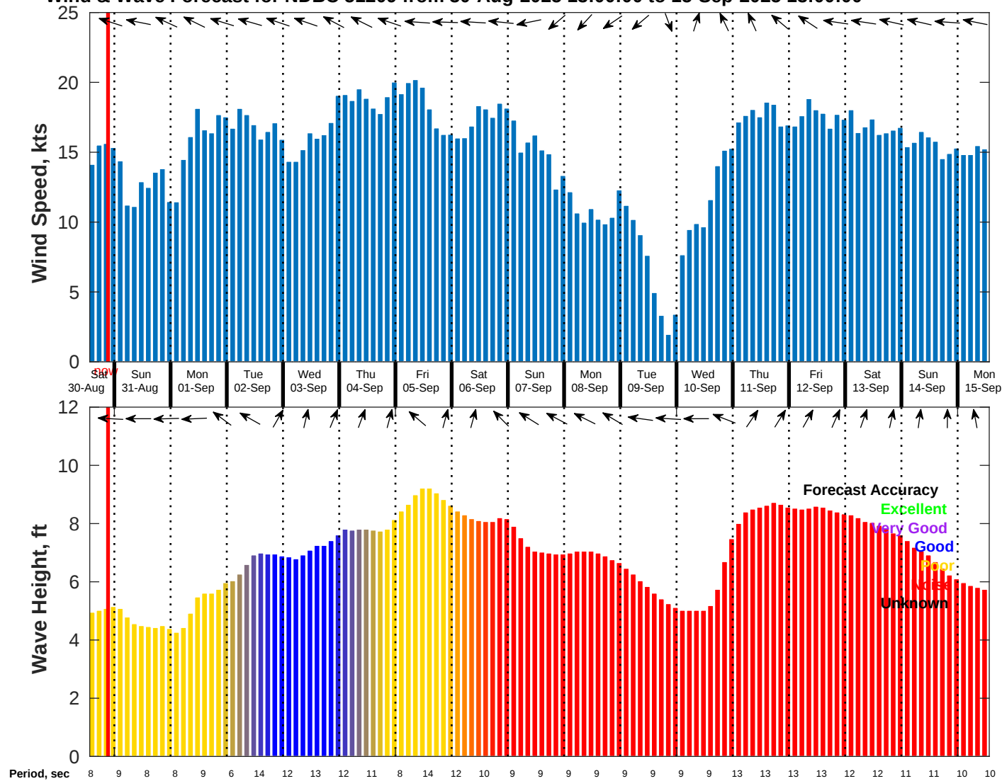
Wind & Wave Forecast for NDBC 51209 from 30-Aug-2025 13:00:00 to 15-Sep-2025 13:00:00
