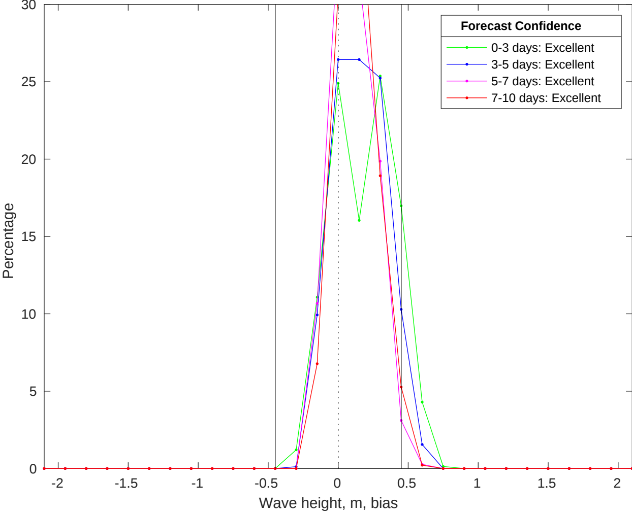
NDBC 51211 vs CMEMS Waves Bias Histogram: 31-Aug-2025
