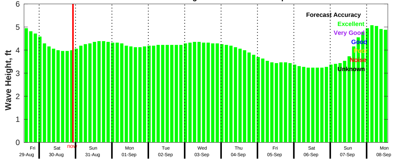
CMEMS Wave Forecast for NDBC 51211 from 29-Aug-2025 14:00:00 to 08-Sep-2025 14:00:00
