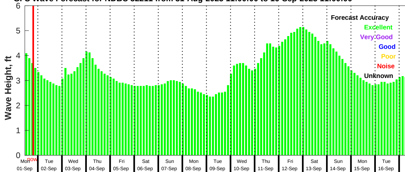
GFS Wave Forecast for NDBC 52211 from 31-Aug-2025 11:00:00 to 16-Sep-2025 11:00:00
