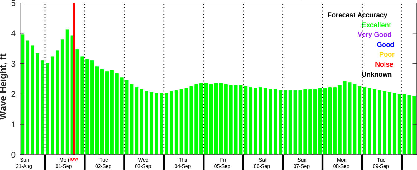
CMEMS Wave Forecast for NDBC 52212 from 30-Aug-2025 09:00:00 to 09-Sep-2025 09:00:00
