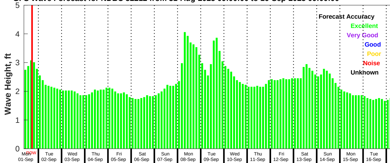
GFS Wave Forecast for NDBC 52212 from 31-Aug-2025 09:00:00 to 16-Sep-2025 09:00:00
