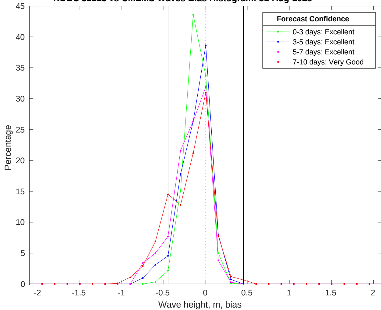
NDBC 52213 vs CMEMS Waves Bias Histogram: 31-Aug-2025
