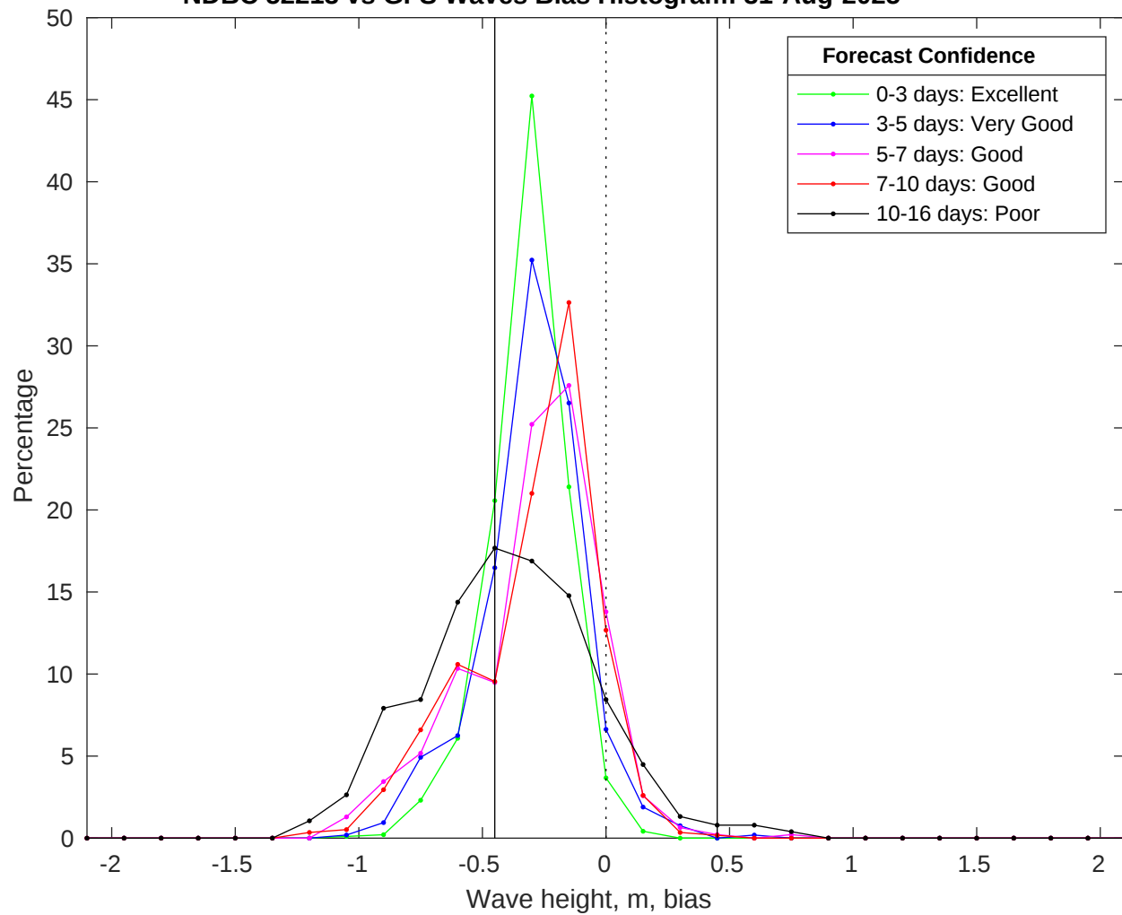
NDBC 52213 vs GFS Waves Bias Histogram: 31-Aug-2025
