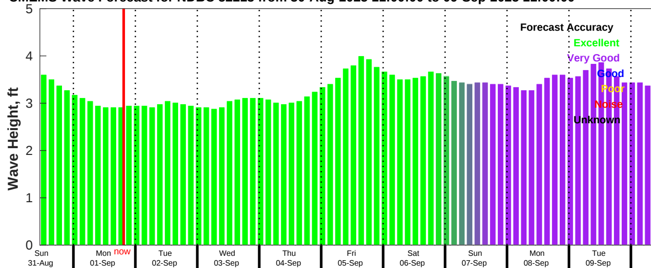
CMEMS Wave Forecast for NDBC 52213 from 30-Aug-2025 11:00:00 to 09-Sep-2025 11:00:00
