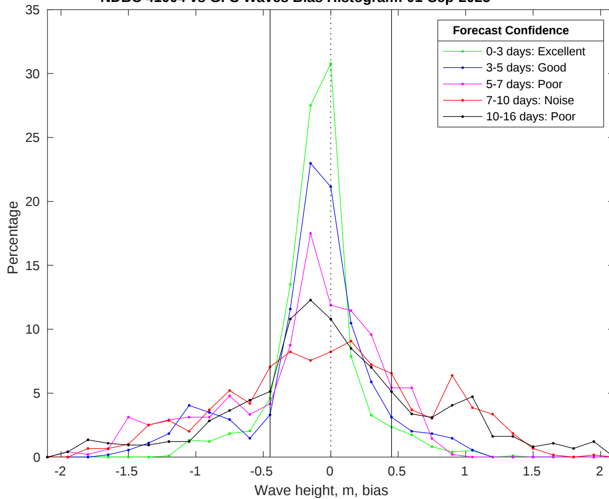
NDBC 41004 vs GFS Waves Bias Histogram: 01-Sep-2025
