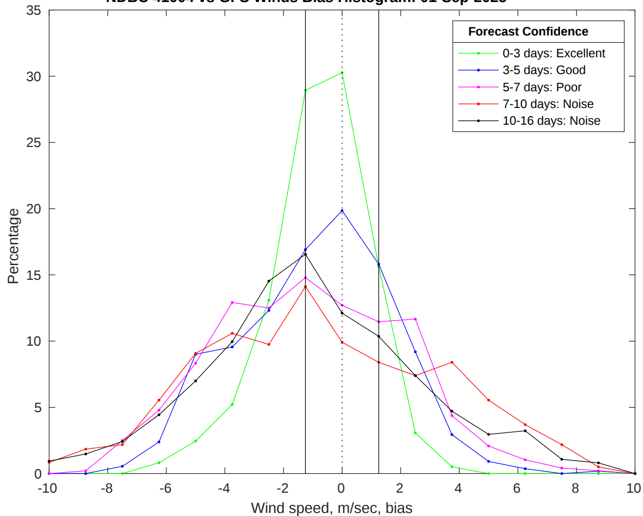
NDBC 41004 vs GFS Winds Bias Histogram: 01-Sep-2025
