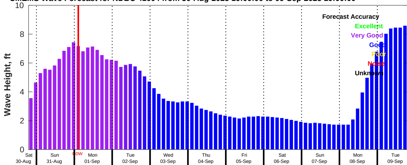
CMEMS Wave Forecast for NDBC 41004 from 30-Aug-2025 19:00:00 to 09-Sep-2025 19:00:00
