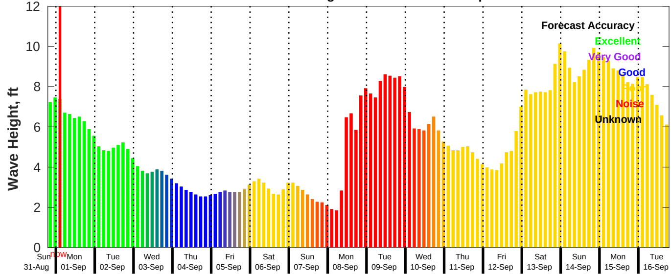
GFS Wave Forecast for NDBC 41004 from 31-Aug-2025 19:00:00 to 16-Sep-2025 19:00:00
