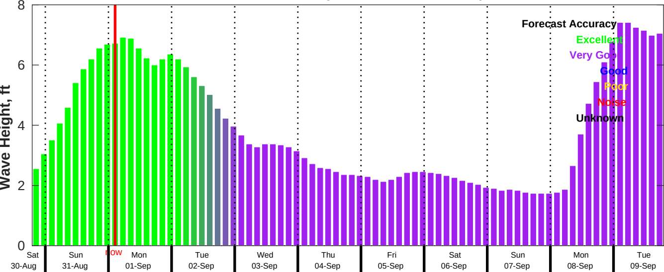
CMEMS Wave Forecast for NDBC 41013 from 30-Aug-2025 19:00:00 to 09-Sep-2025 19:00:00
