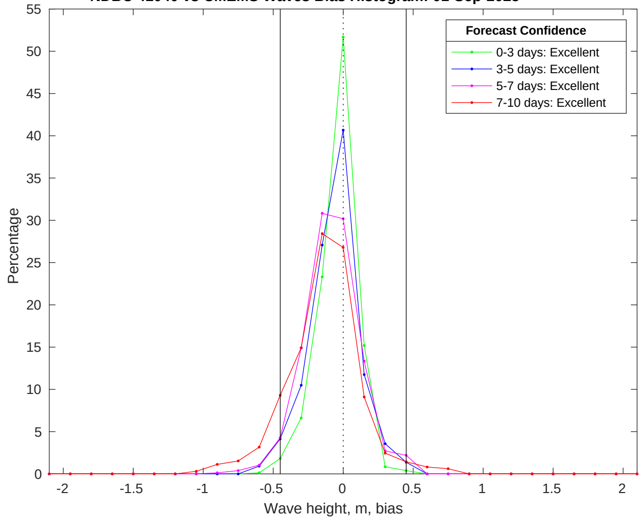
NDBC 41040 vs CMEMS Waves Bias Histogram: 01-Sep-2025
