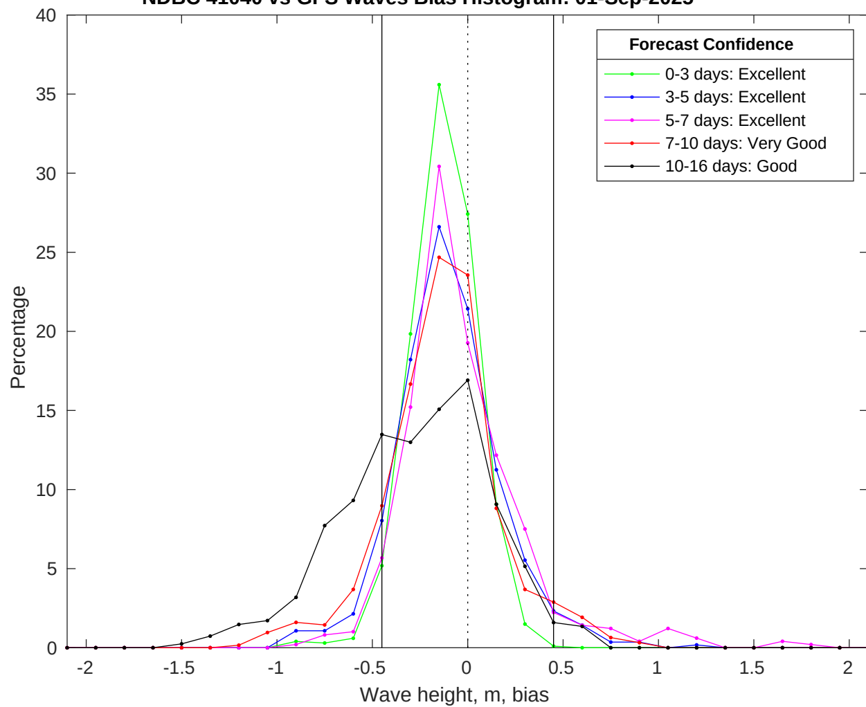
NDBC 41040 vs GFS Waves Bias Histogram: 01-Sep-2025
