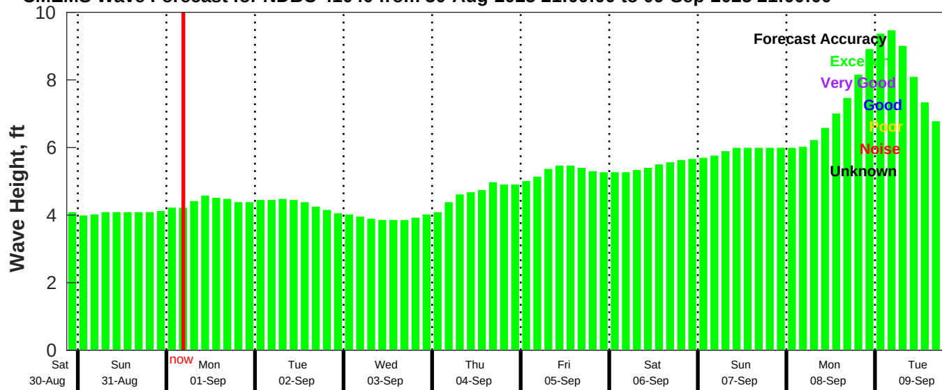
CMEMS Wave Forecast for NDBC 41040 from 30-Aug-2025 21:00:00 to 09-Sep-2025 21:00:00
