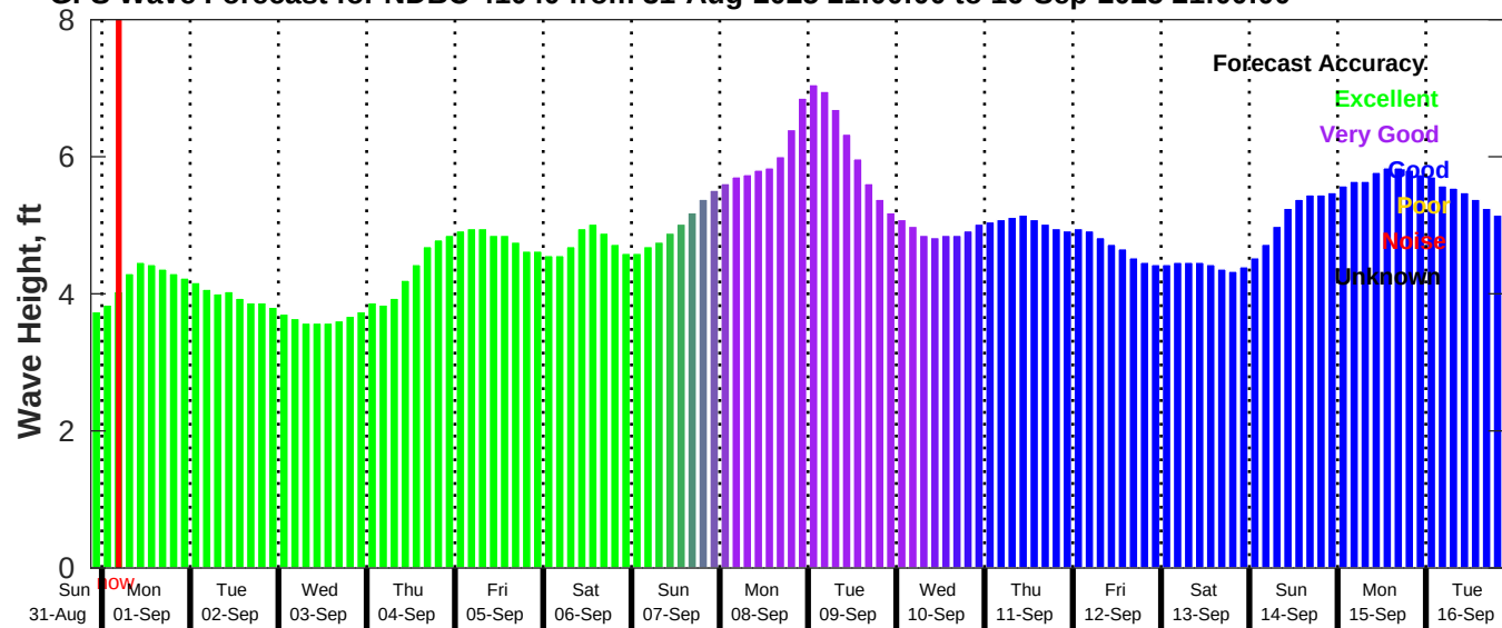
GFS Wave Forecast for NDBC 41040 from 31-Aug-2025 21:00:00 to 16-Sep-2025 21:00:00
