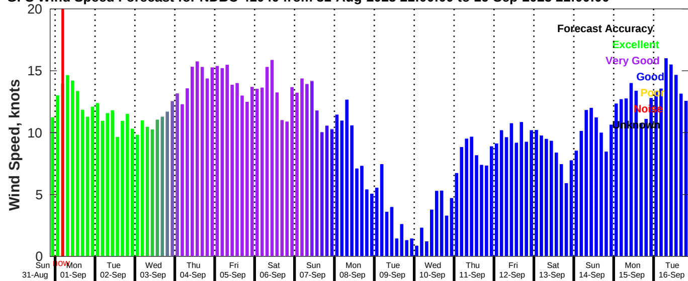
GFS Wind Speed Forecast for NDBC 41040 from 31-Aug-2025 21:00:00 to 16-Sep-2025 21:00:00
