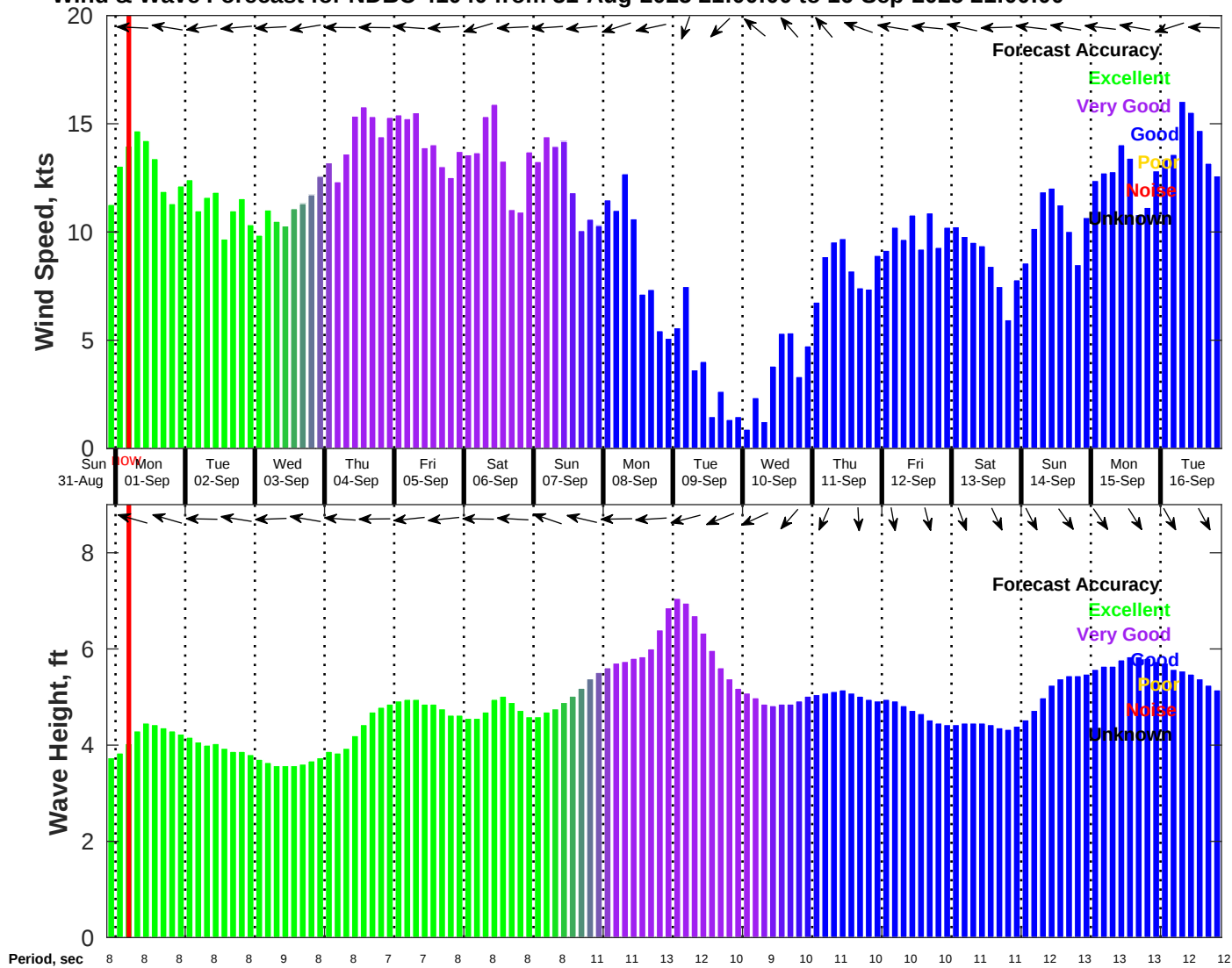
Wind & Wave Forecast for NDBC 41040 from 31-Aug-2025 21:00:00 to 16-Sep-2025 21:00:00
