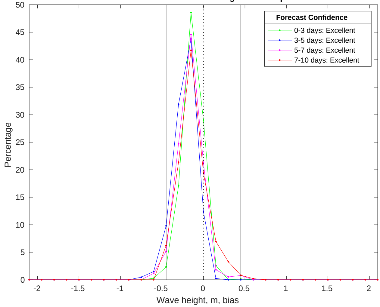
NDBC 42019 vs CMEMS Waves Bias Histogram: 01-Sep-2025
