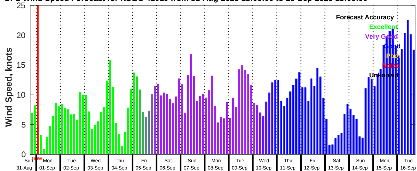
GFS Wind Speed Forecast for NDBC 42019 from 31-Aug-2025 18:00:00 to 16-Sep-2025 18:00:00
