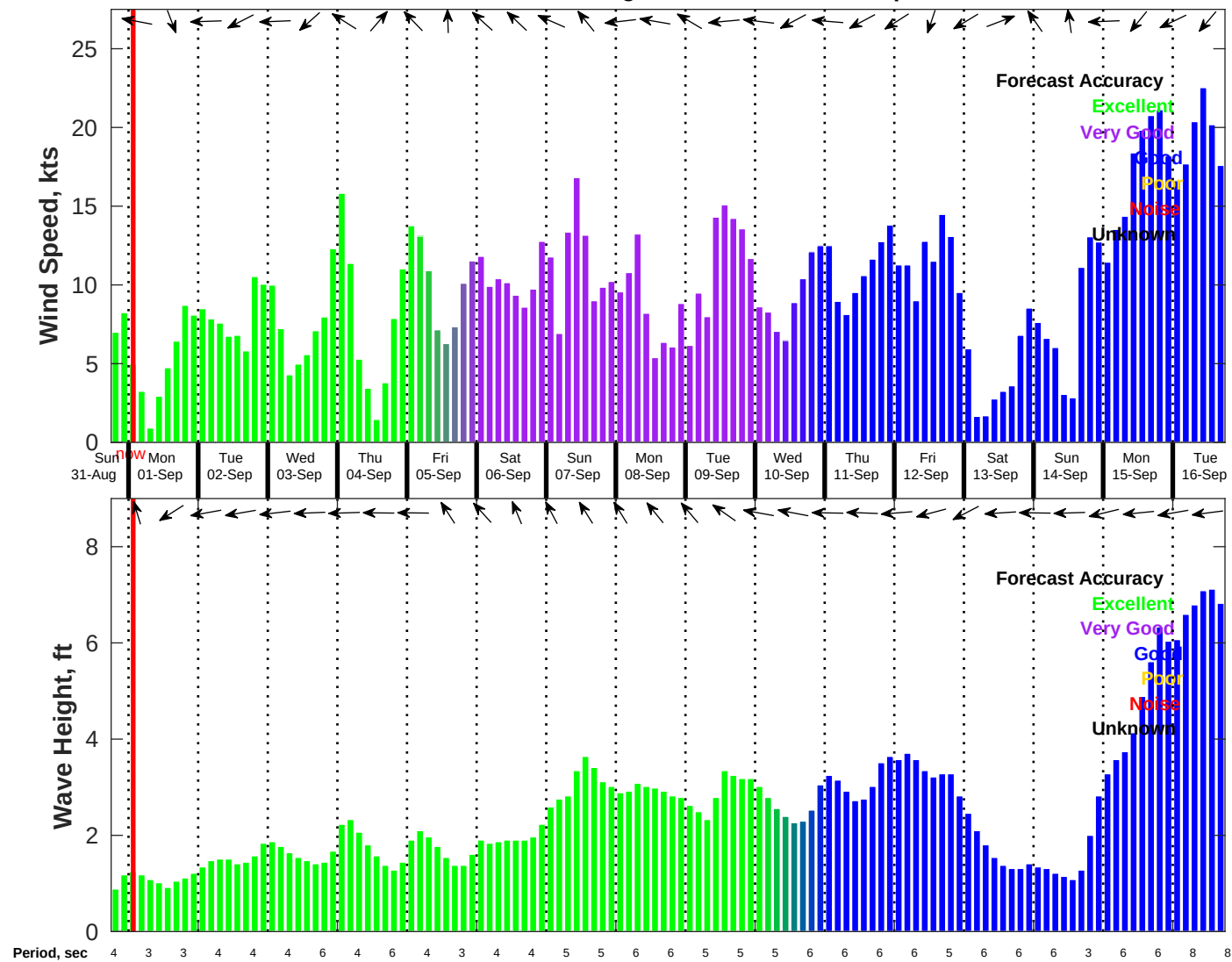
Wind & Wave Forecast for NDBC 42019 from 31-Aug-2025 18:00:00 to 16-Sep-2025 18:00:00
