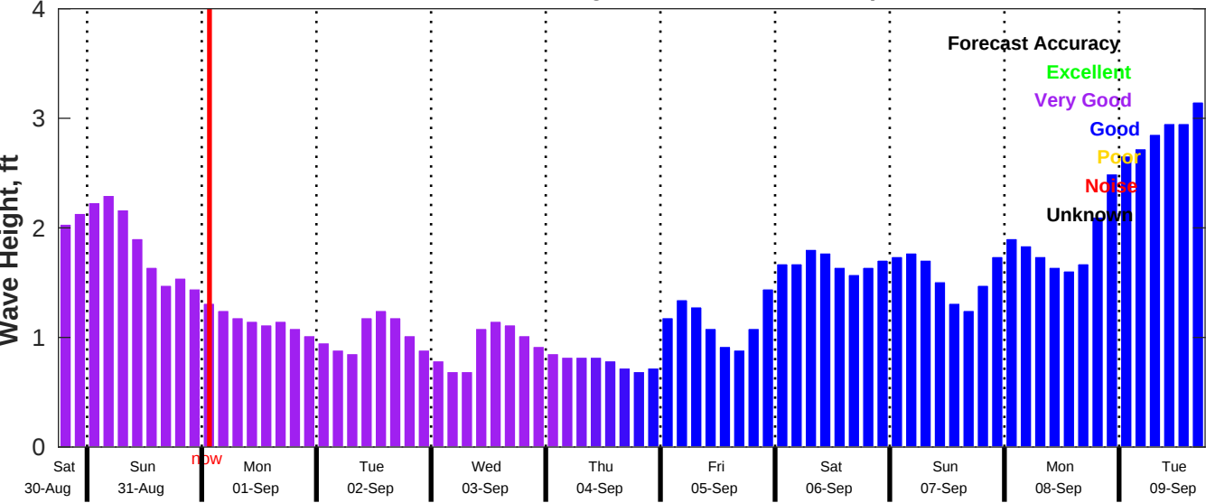
CMEMS Wave Forecast for NDBC 42020 from 30-Aug-2025 18:00:00 to 09-Sep-2025 18:00:00
