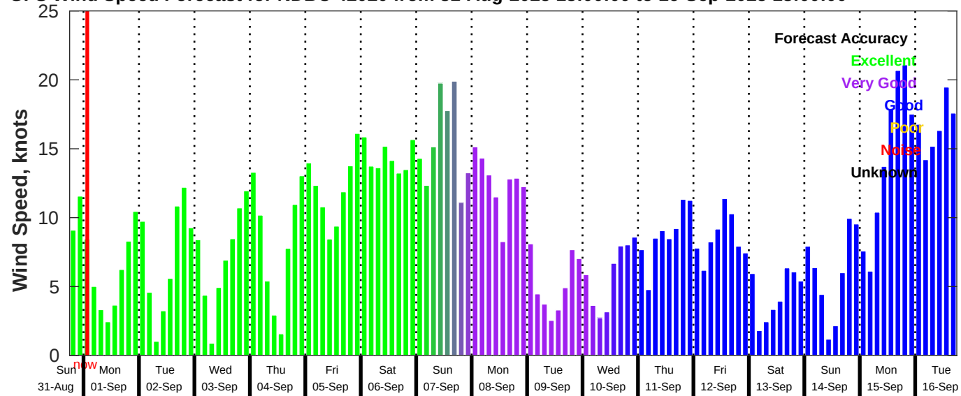
GFS Wind Speed Forecast for NDBC 42020 from 31-Aug-2025 18:00:00 to 16-Sep-2025 18:00:00
