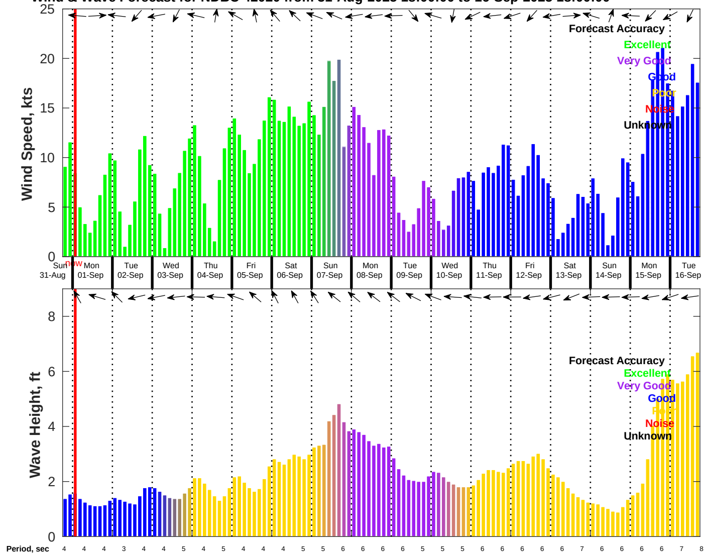
Wind & Wave Forecast for NDBC 42020 from 31-Aug-2025 18:00:00 to 16-Sep-2025 18:00:00
