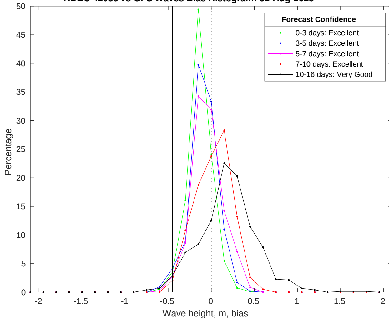
NDBC 42035 vs GFS Waves Bias Histogram: 31-Aug-2025
