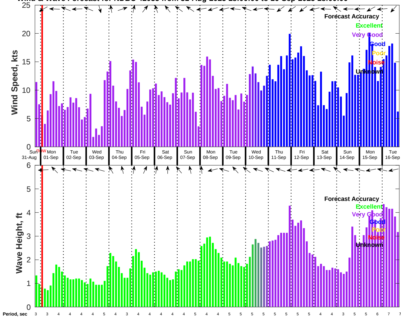
Wind & Wave Forecast for NDBC 42035 from 31-Aug-2025 18:00:00 to 16-Sep-2025 18:00:00
