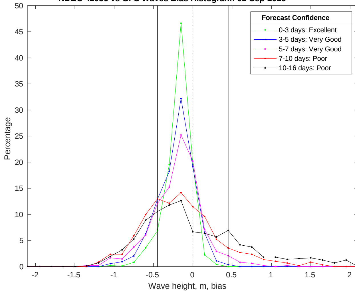
NDBC 42036 vs GFS Waves Bias Histogram: 01-Sep-2025
