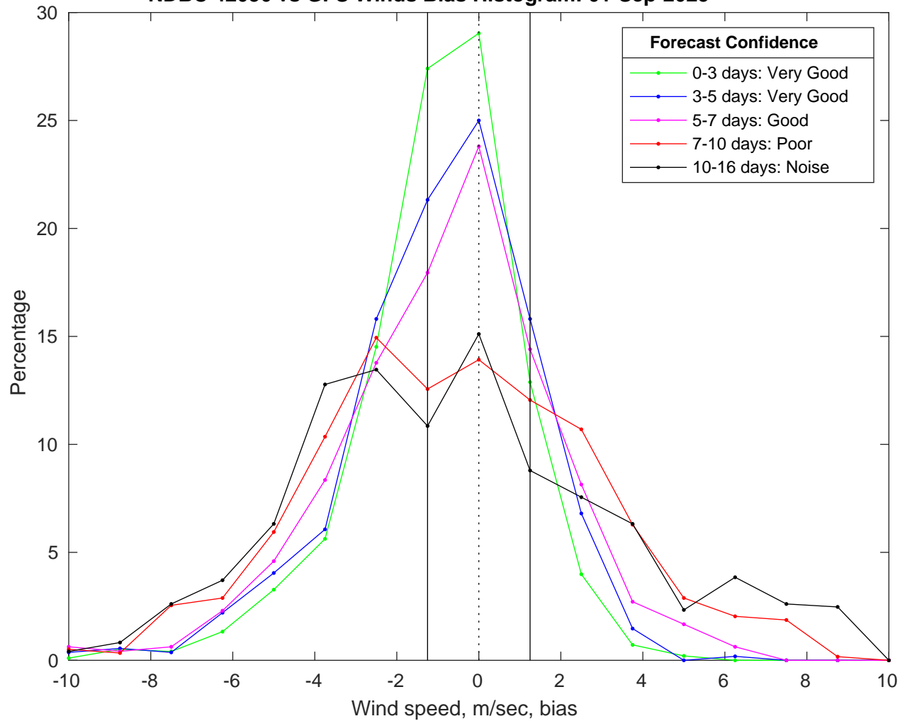
NDBC 42036 vs GFS Winds Bias Histogram: 01-Sep-2025
