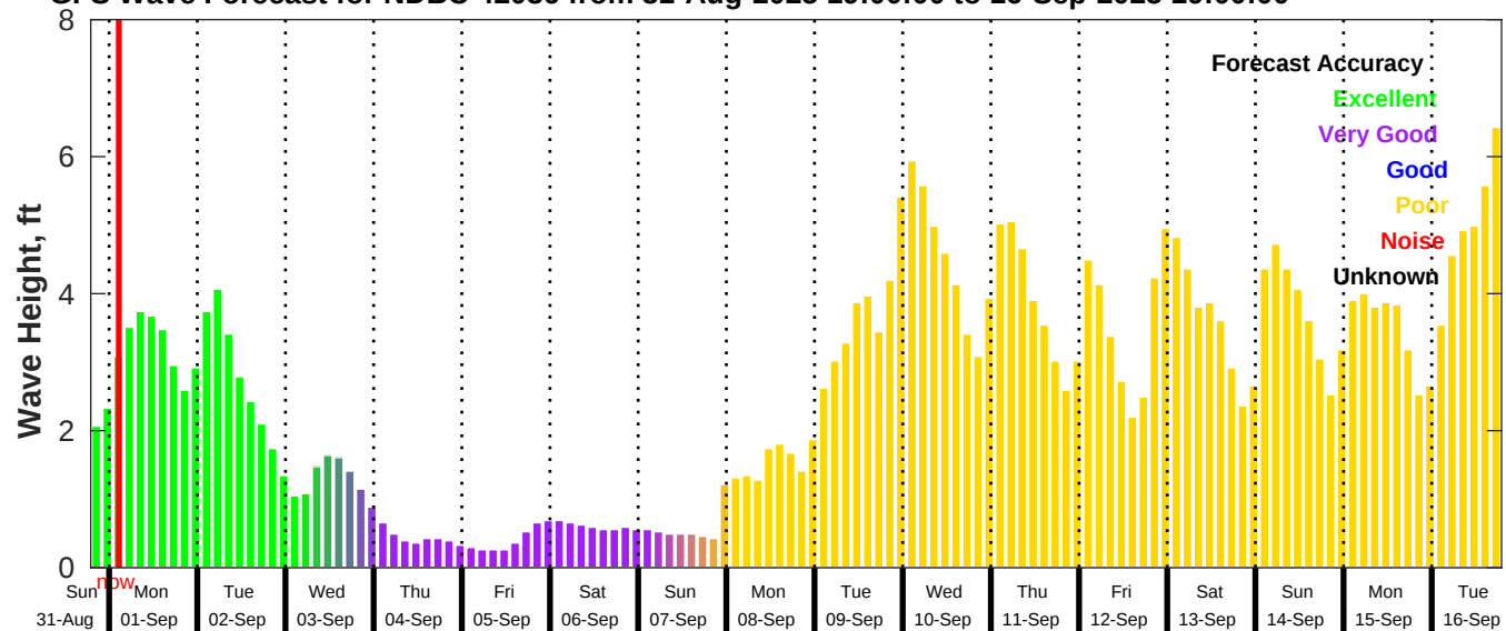
GFS Wave Forecast for NDBC 42036 from 31-Aug-2025 19:00:00 to 16-Sep-2025 19:00:00
