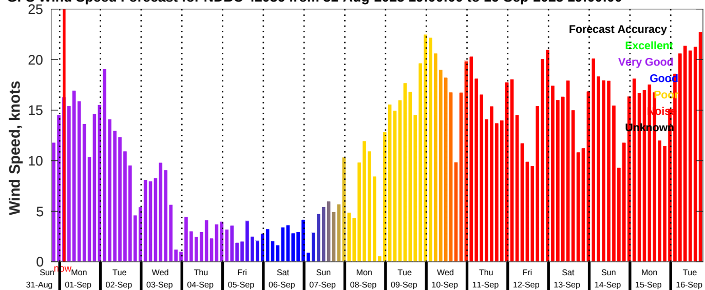
GFS Wind Speed Forecast for NDBC 42036 from 31-Aug-2025 19:00:00 to 16-Sep-2025 19:00:00
