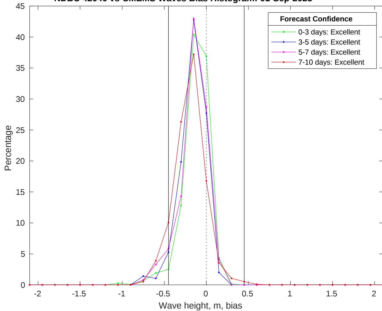
NDBC 42040 vs CMEMS Waves Bias Histogram: 01-Sep-2025
