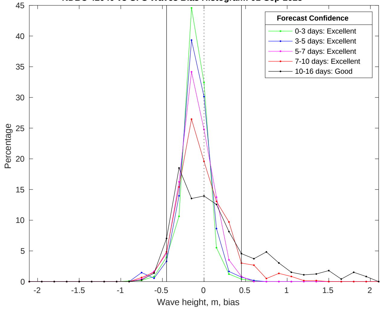
NDBC 42040 vs GFS Waves Bias Histogram: 01-Sep-2025
